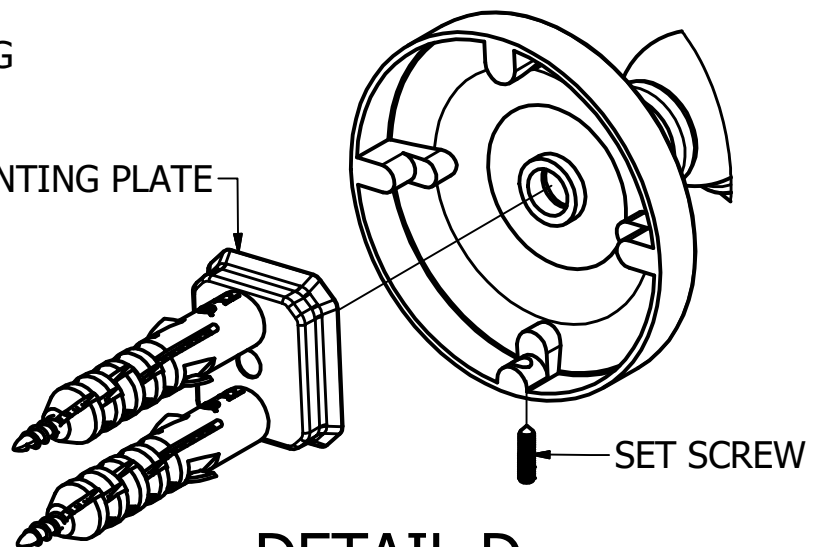
DETAIL D
