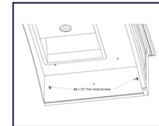
Step 6: Fasten wood range hood to liner with (4) screws
