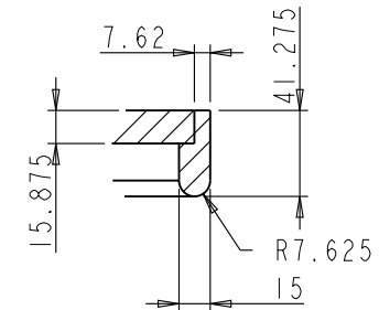
DETAIL A SCALE 1:4
