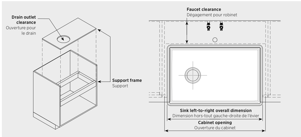
IMAGE 1 SUPPORT FRAME AND CLEARANCE / SUPPORT ET DÉGAGEMENT
