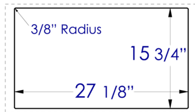
Counter Top Cut Out
