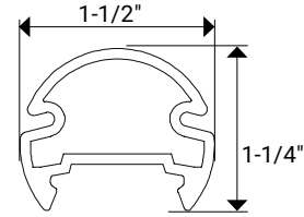
Fixture Cross-Section
