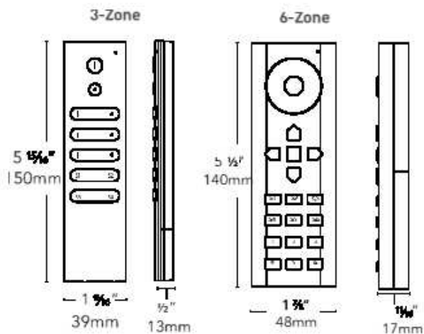
3-Zone (CR2032)
