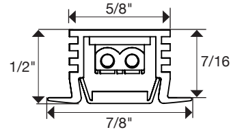
Fixture Cross-Section
