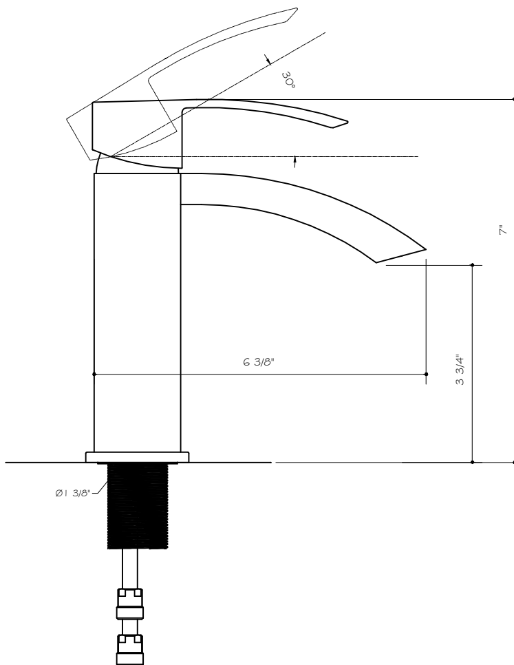
SIDE VIEW
