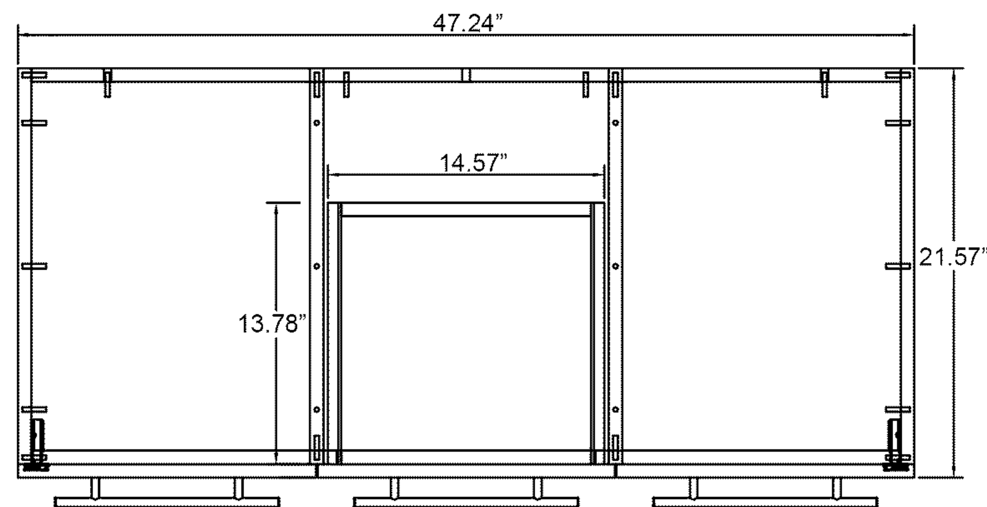
Top View
