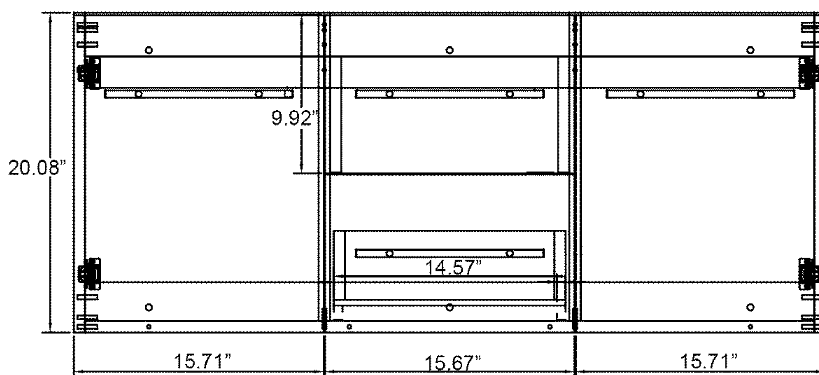
Front View
