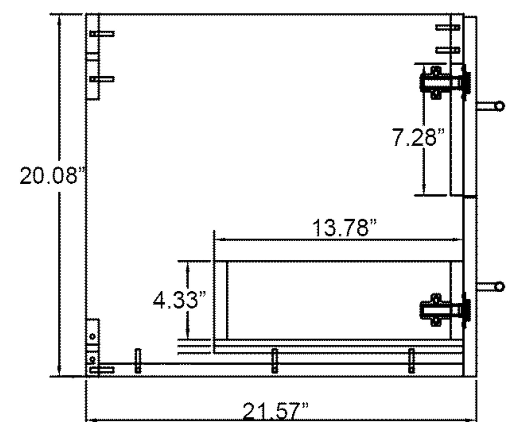
Side View
