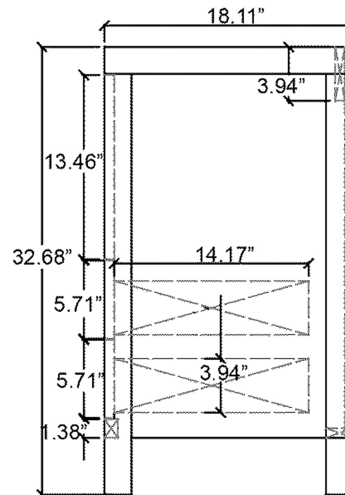
Side View
