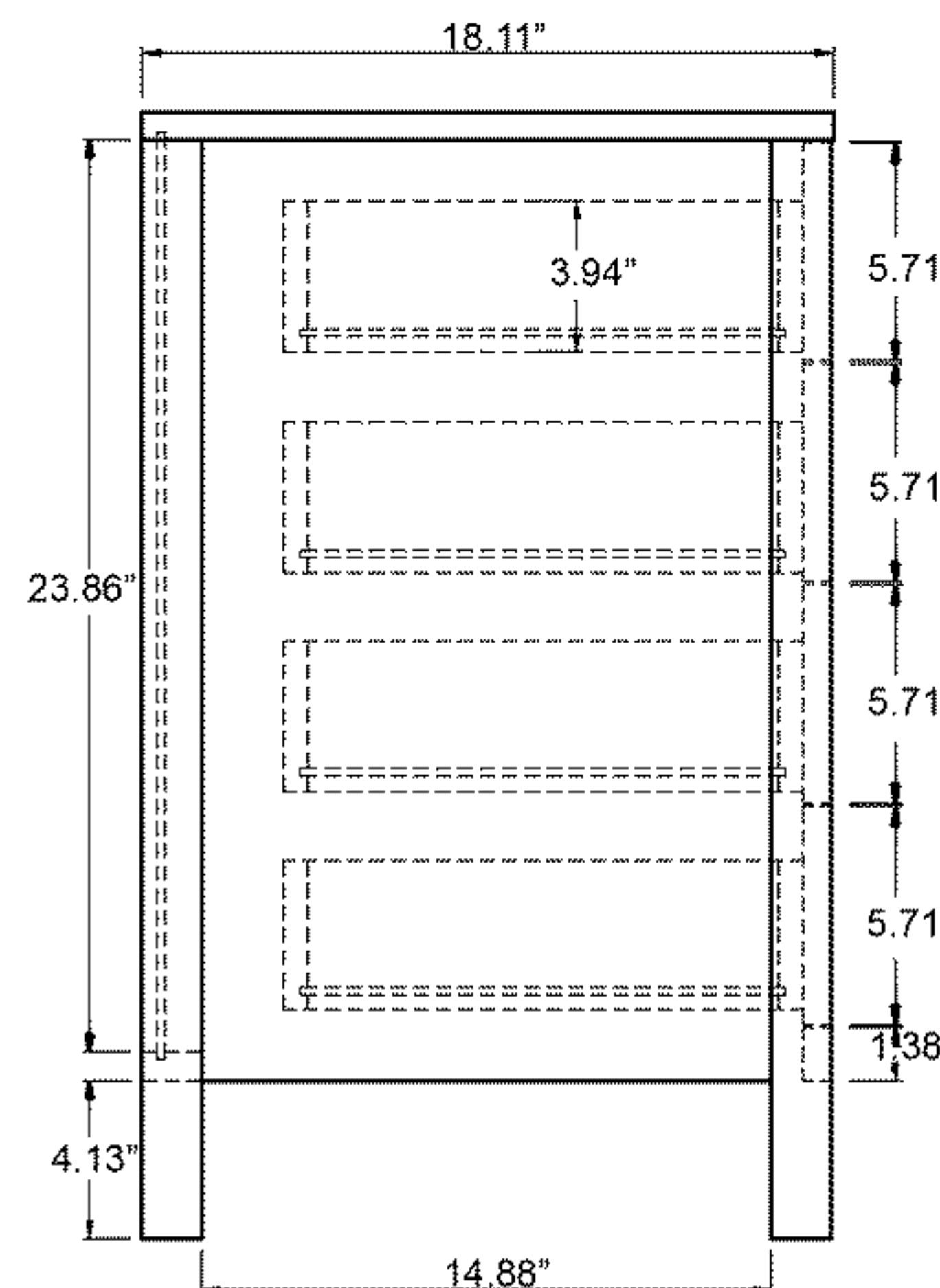
Side View
