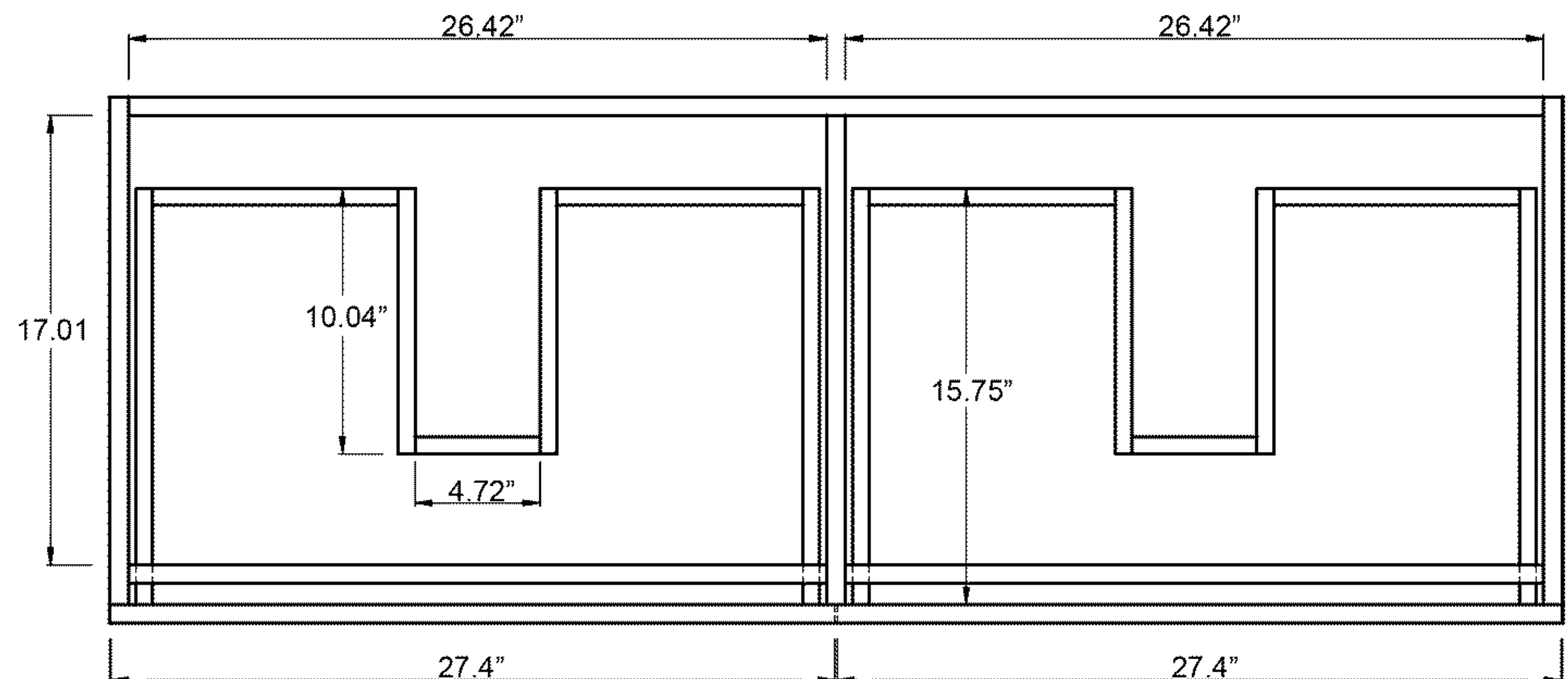
Top View
