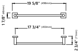
Model #: KEA-17736 Towel Bar Dimensions: 19\frac{5}{8}'' \times 2\frac{3}{4}'' \times 1\frac{7}{8}''
