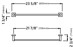
Model #: KEA-17737 Towel Bar Dimensions: 23\frac{5}{8}'' \times 2\frac{3}{4}'' \times 1\frac{3}{4}''
