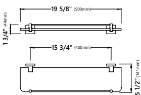
Model #: KEA-17745 Bathroom Shelf Dimensions: 19\frac{5}{8}'' \times 5\frac{1}{2}'' \times 1\frac{3}{4}''
