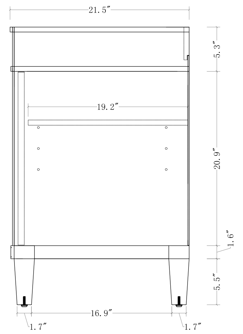
SIDE VIEW
