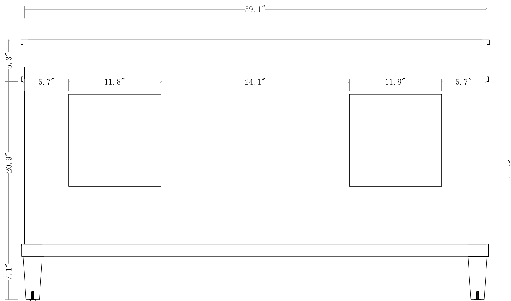
BACK VIEW
