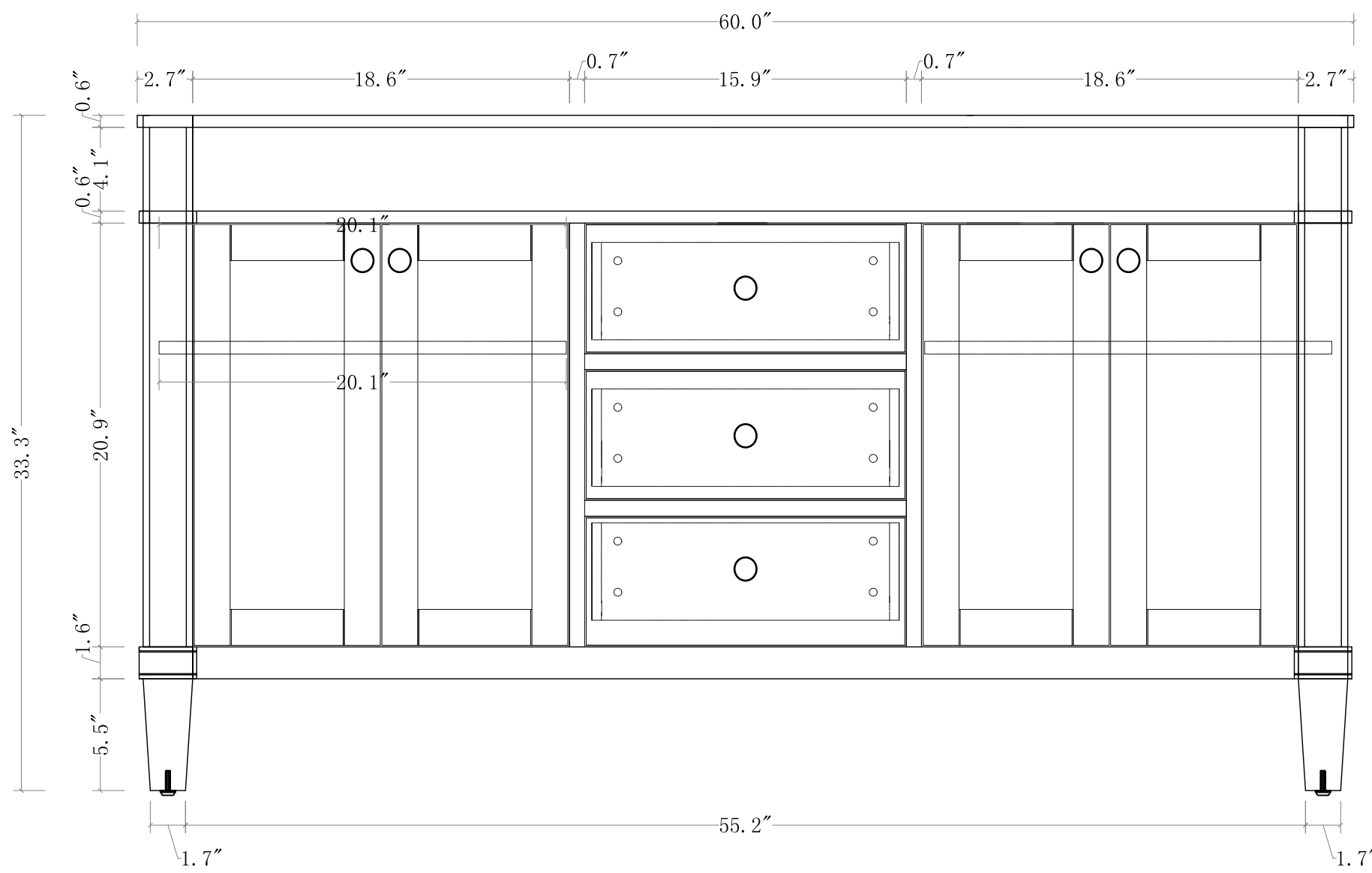
FRONT VIEW
