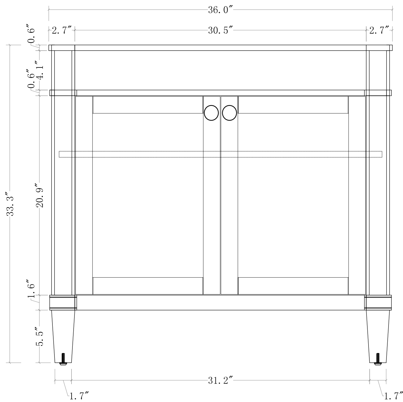
FRONT VIEW
