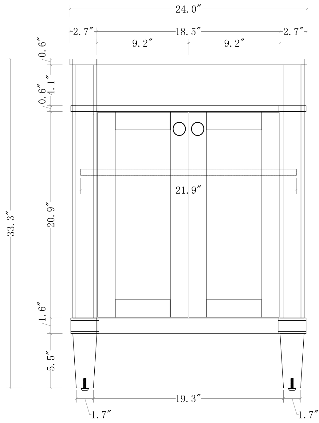
FRONT VIEW
