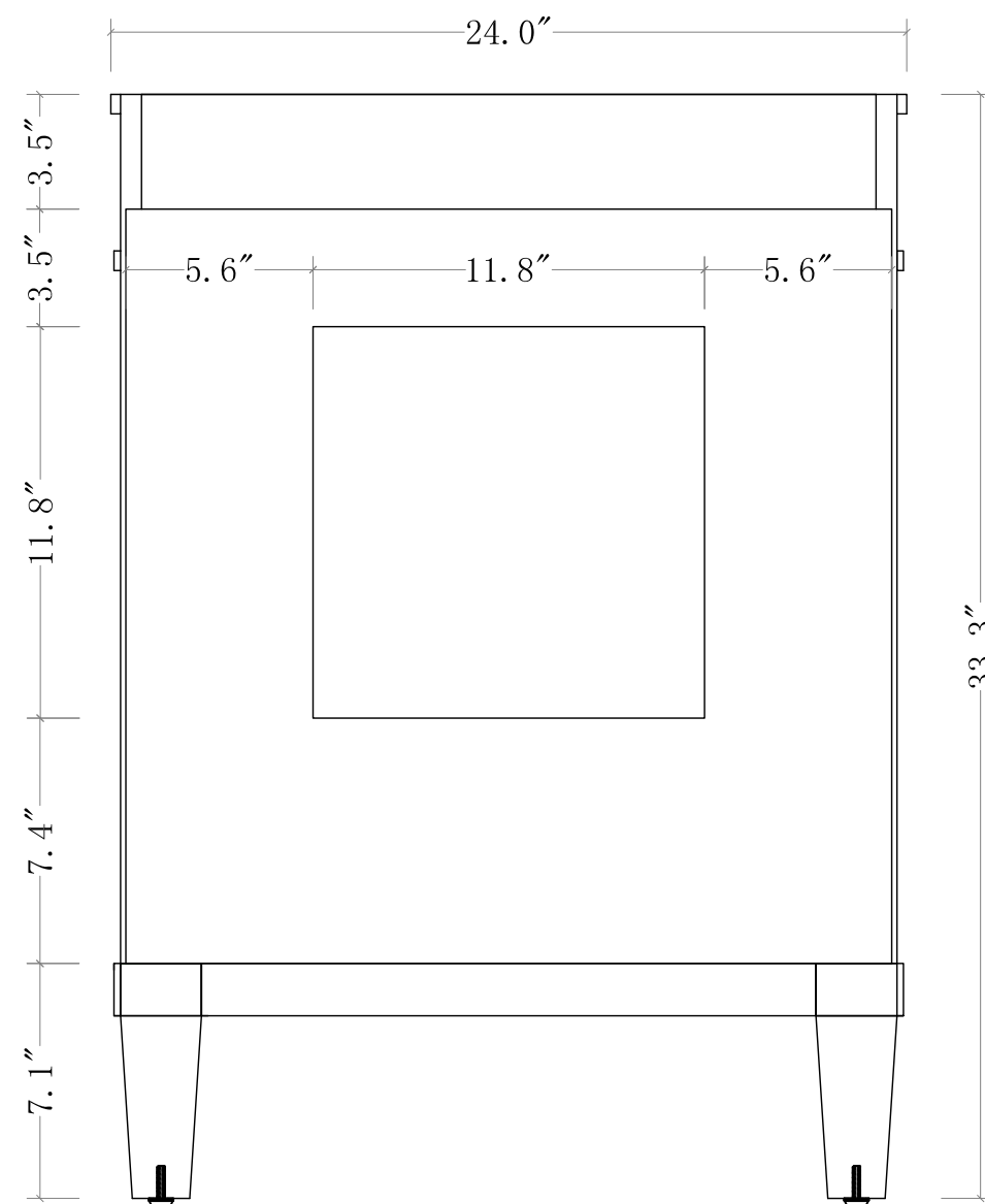
BACK VIEW
