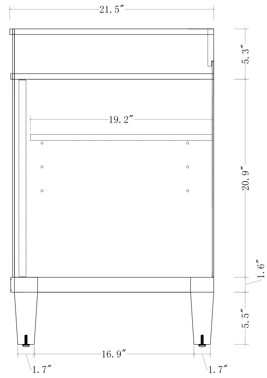
SIDE VIEW
