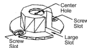
Brass Fitting
