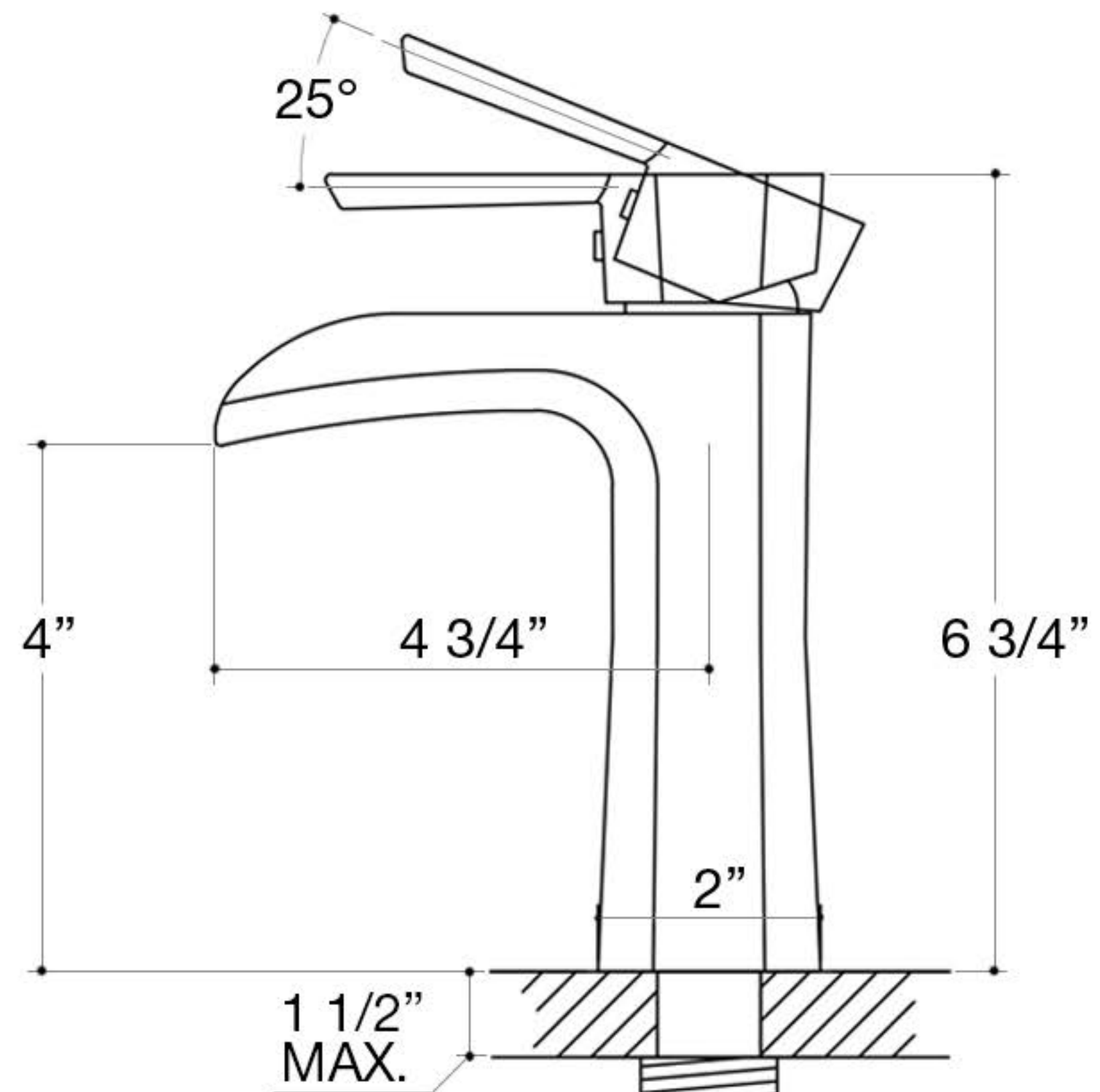
SIDE VIEW
