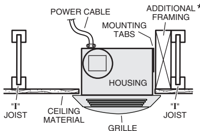
HOUSING MOUNTED TO "1" JOIST Requires additional framing for mounting tabs.
