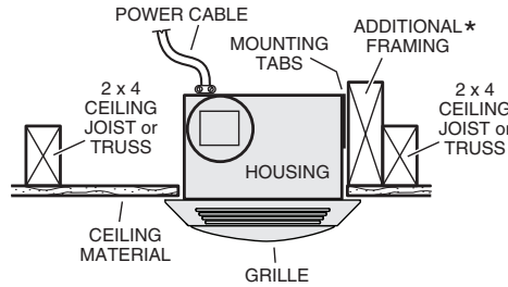
HOUSING MOUNTED TO 2x4 TRUSS Requires additional framing for mounting tabs.
