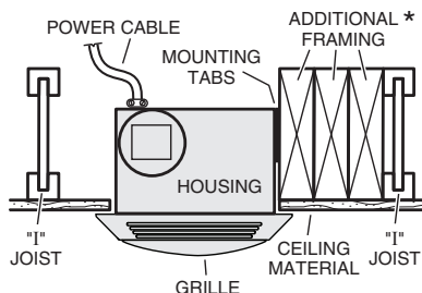
HOUSING MOUNTED IN ANY LOCATION BETWEEN JOISTS Requires additional framing for mounting tabs.
