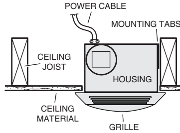
HOUSING MOUNTED DIRECTLY TO JOIST 2x6 (or larger)
