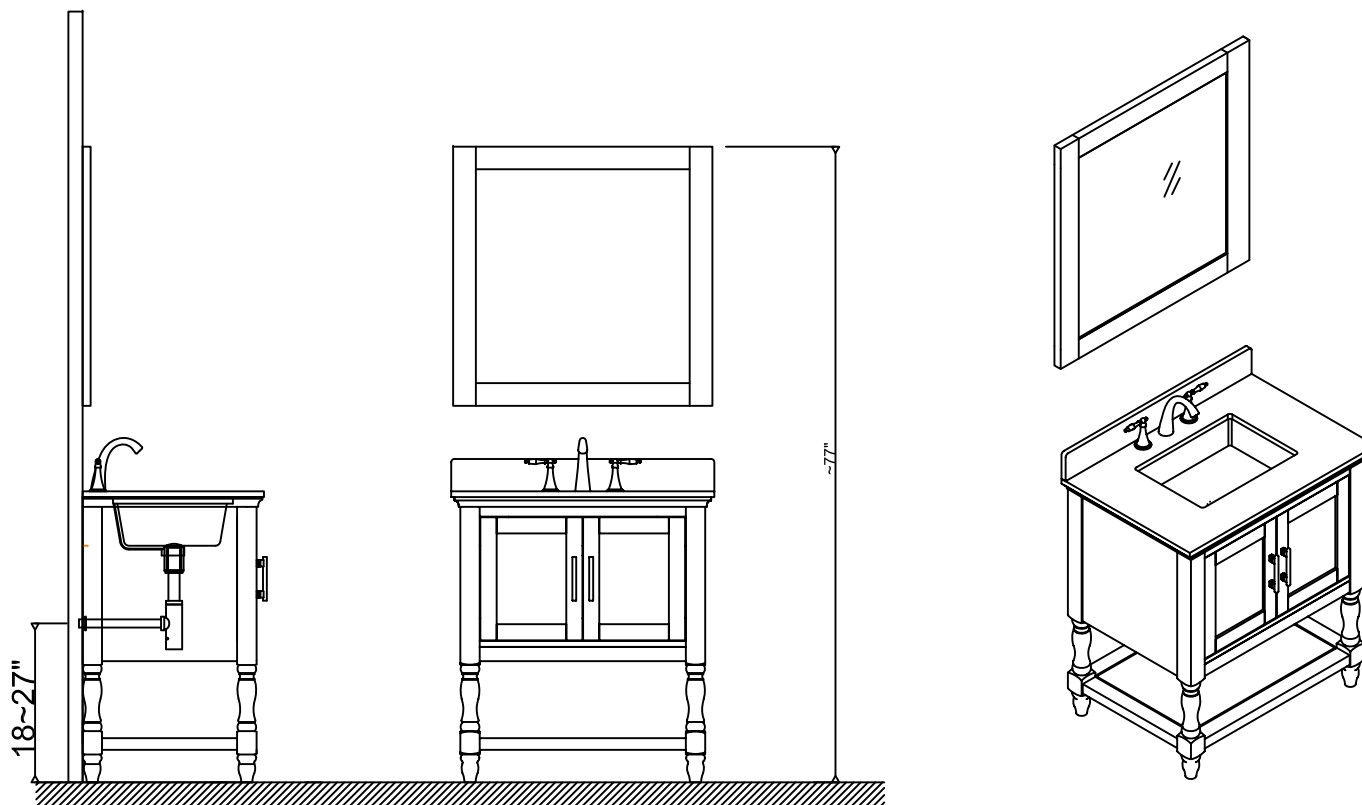
3. Basin
